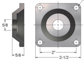
SM-29 FLANGE MOUNT
