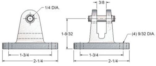
A-139 SWIVEL BRACKET
